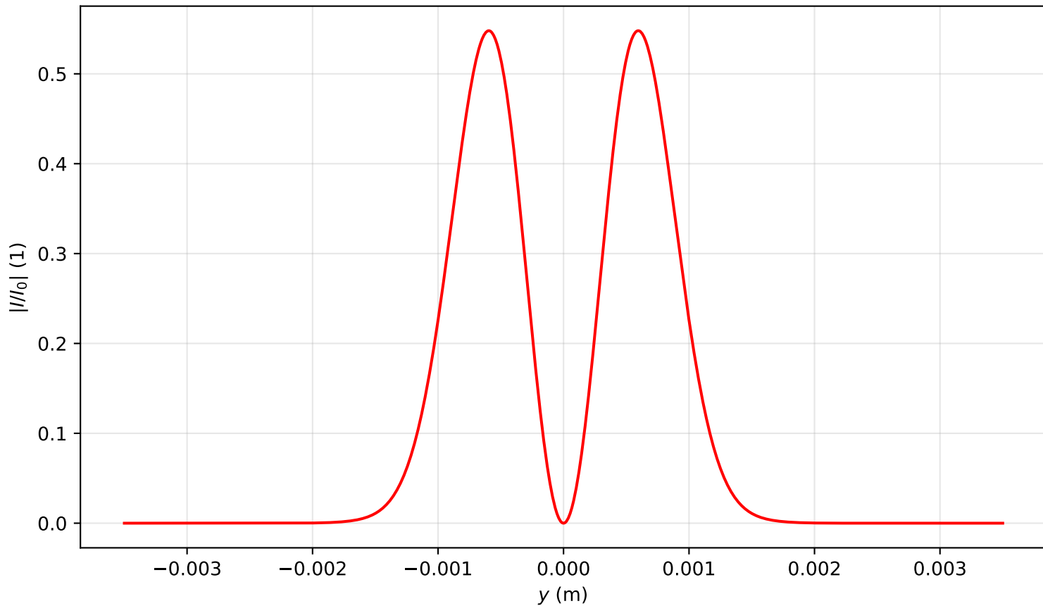
Intensity profile I(x=0, y, z=1.274)/I_0 , P_{in}=0.5P_{cr} , artificial time
